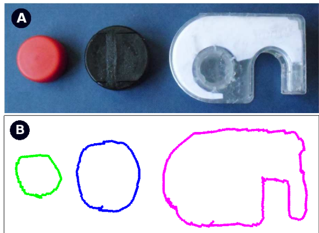
Fig. 8: Traced contours from applying active perception to an online contour following task. (A) Circles with 2 cm, 4 cm diameter and an asymmetric object (sellotape holder) used for real-time contour following. (B) Contours traced obtained as result of active perception applied to sensorimotor control.
